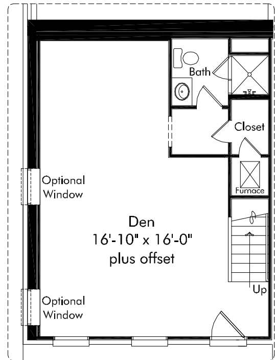
OPTION 2 - ADDS 144 SQ. FT.
