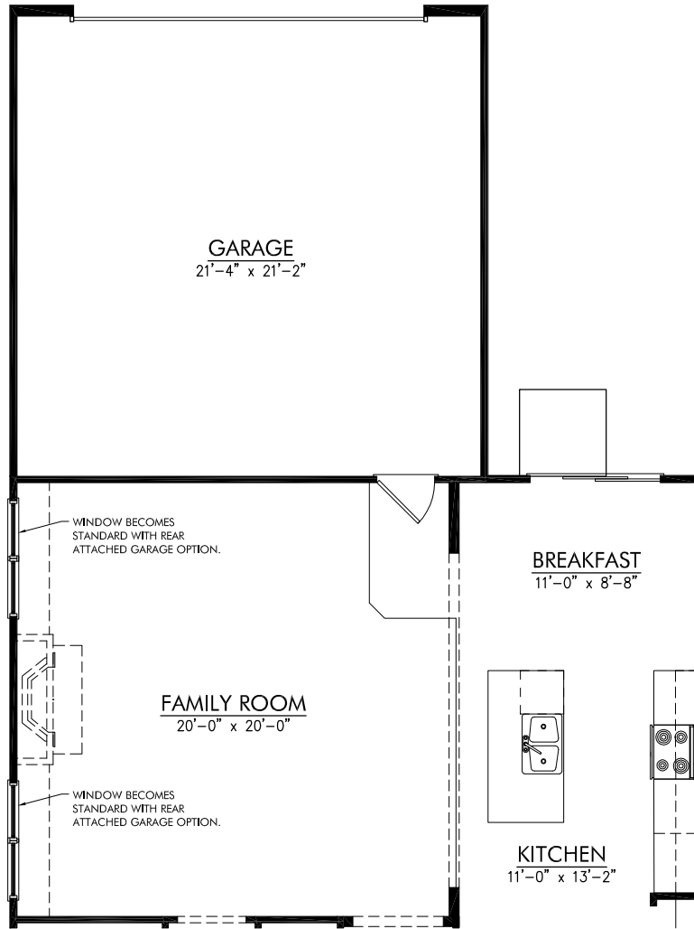
REAR ATTACHED GARAGE OPTION
